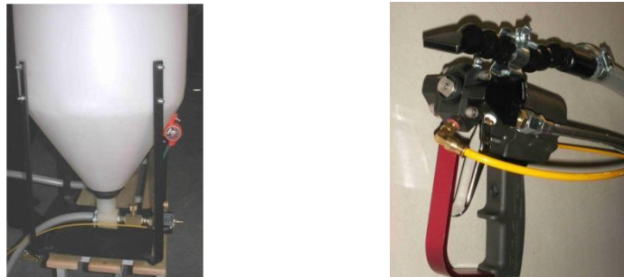
Fig: OL3K Drymix unit; storage (left) and modified spray gun with injector above spray nozzle (right)
